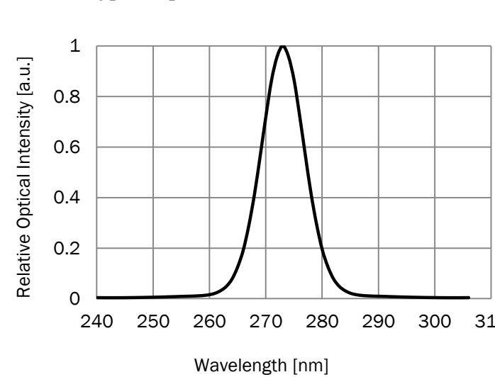
FIG 4. Typical Spectrum
