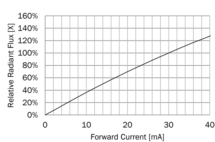
FIG 2. Relative Radiant Flux vs. Forward Current
