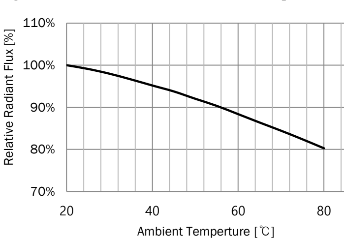
Fig 5. Relative Radiant Flux vs Ambient Temperature
